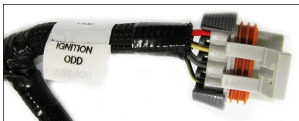
Figure 25 Ignition Odd
