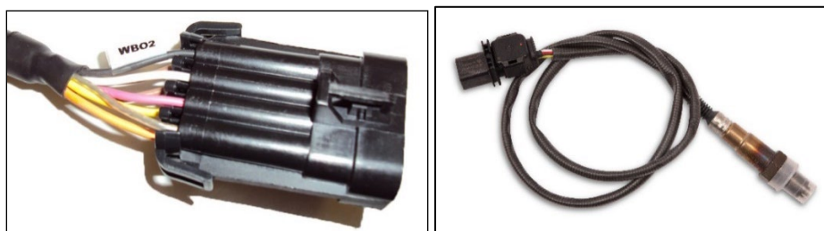
Figure 11 WB02
